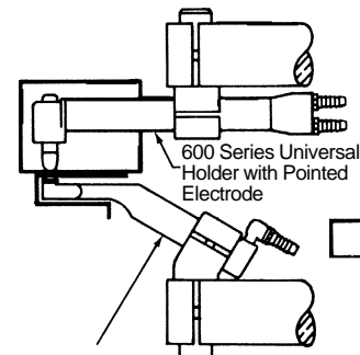
950 Series Paddle Holder with Socket Radius Electrode
